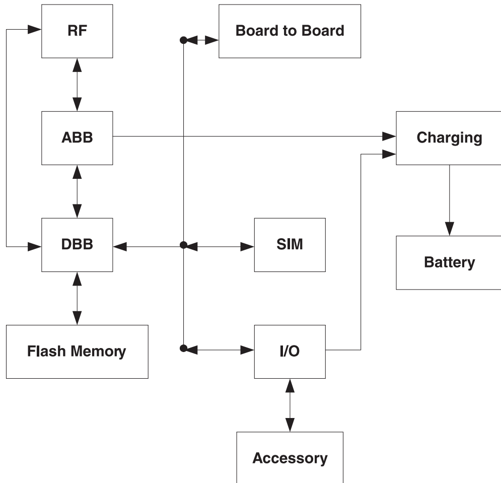
Figure 9-1. Main Block diagram.
